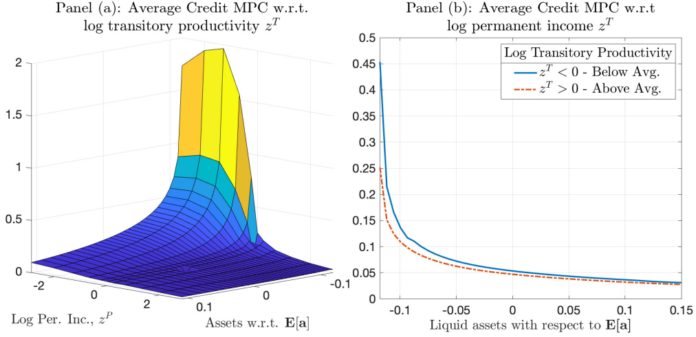
Figure 3.3: Calibrated Distributions of Credit MPCs
