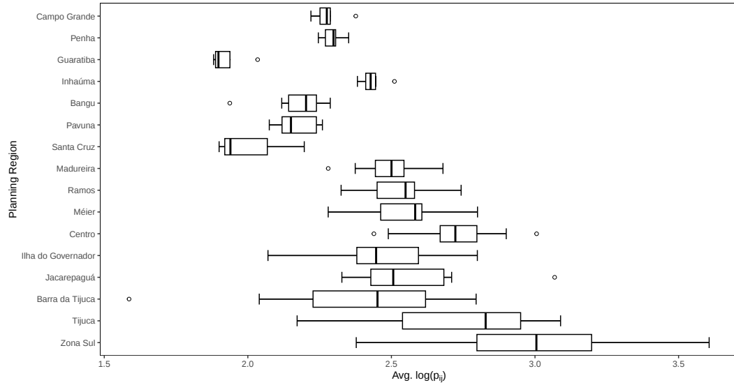
(b) \bar{p}_i^{\text{geom}}
