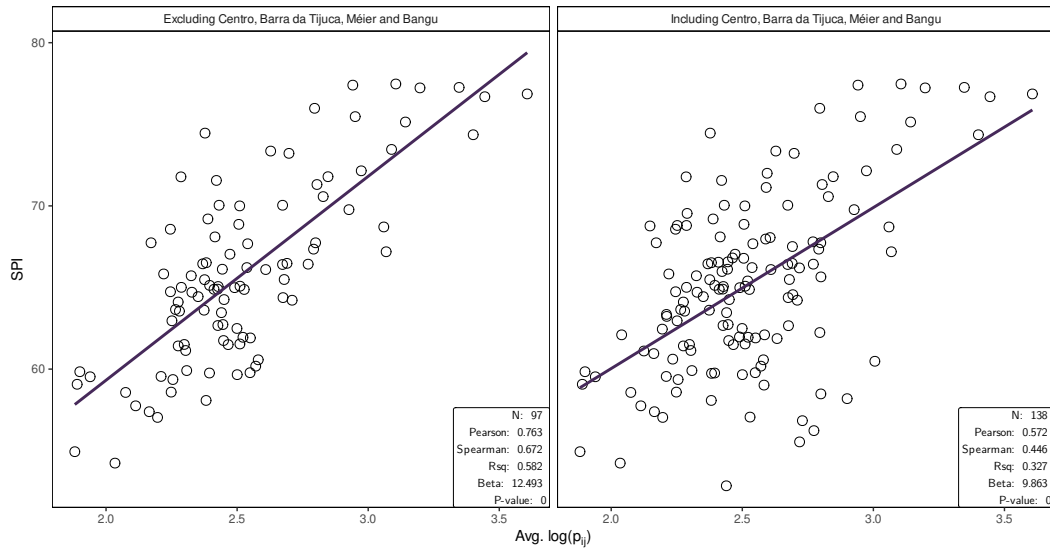
Figure A.1: \text{Avg. log}(p_{ij}) \times \text{SPI} - Excluding outliers
