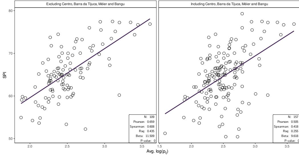
Figure 2.7: \text{Avg. log}(p_{ij}) \times \text{SPI}
