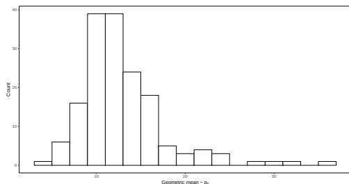
(c) \bar{p}_i^{\text{geom}}
