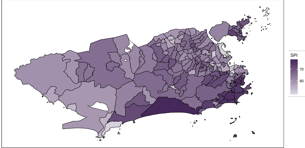
(a) SPI distribution by neighborhoods
