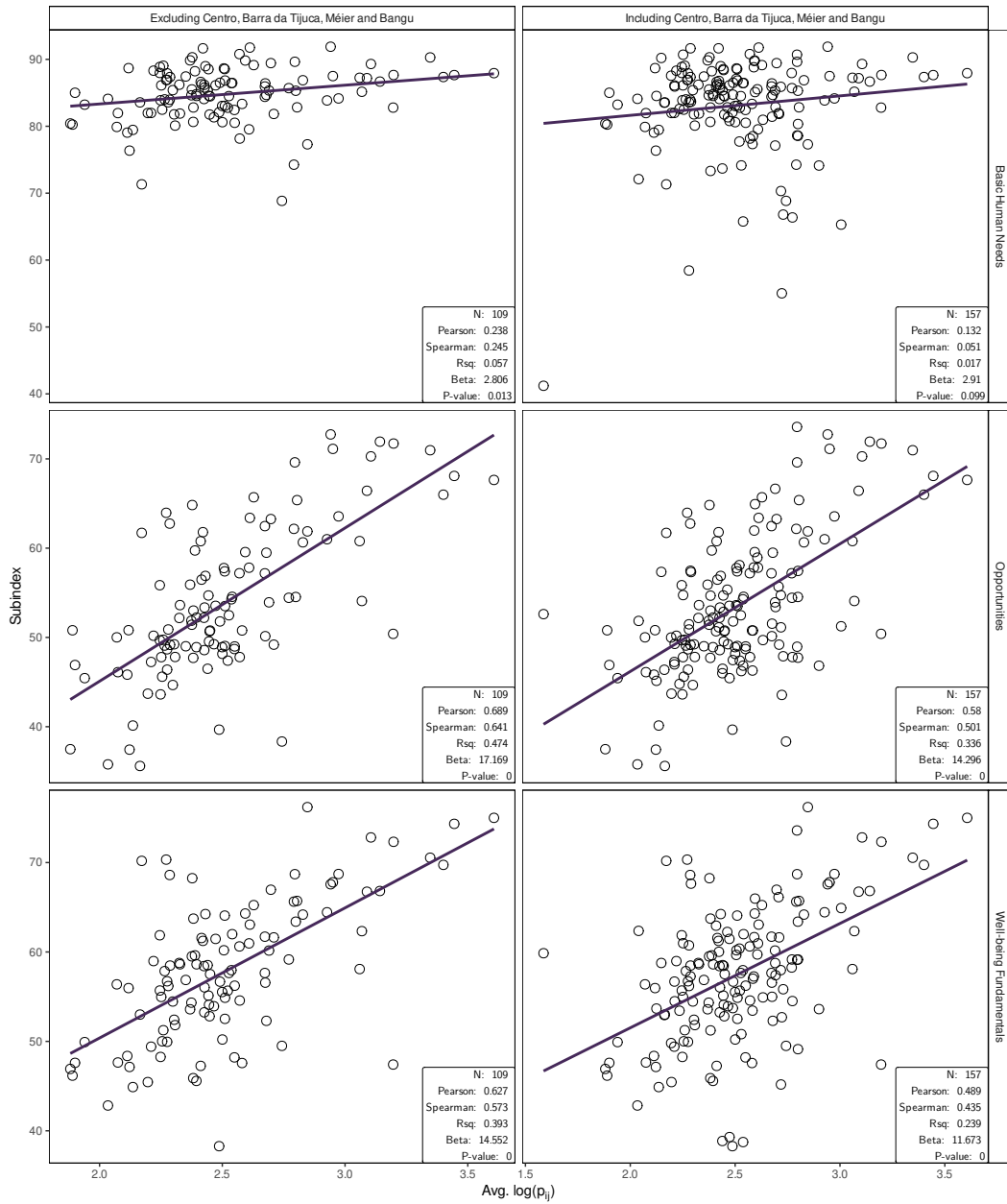
Figure A.4: \text{Avg. log}(p_{ij}) \times \text{SPI} - \text{Subindex decomposition}
