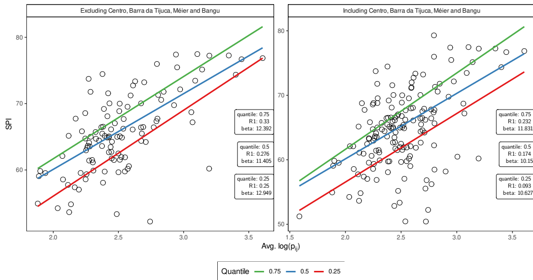
Figure A.2: \text{Avg. log}(p_{ij}) \times \text{SPI} - Quantile regression
