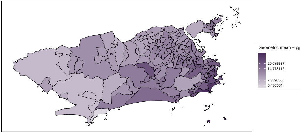
(b) \bar{p}_i^{\text{geom}} distribution by neighborhoods
