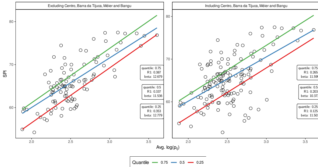
Figure A.3: \text{Avg. log}(p_{ij}) \times \text{SPI} - Quantile regression - Excluding outliers
