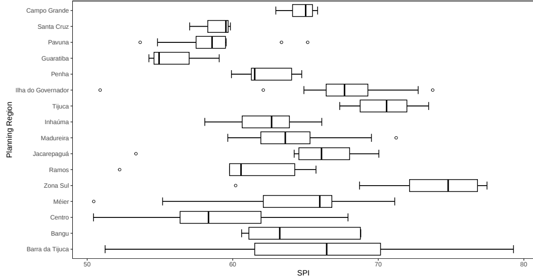
(a) SPI
