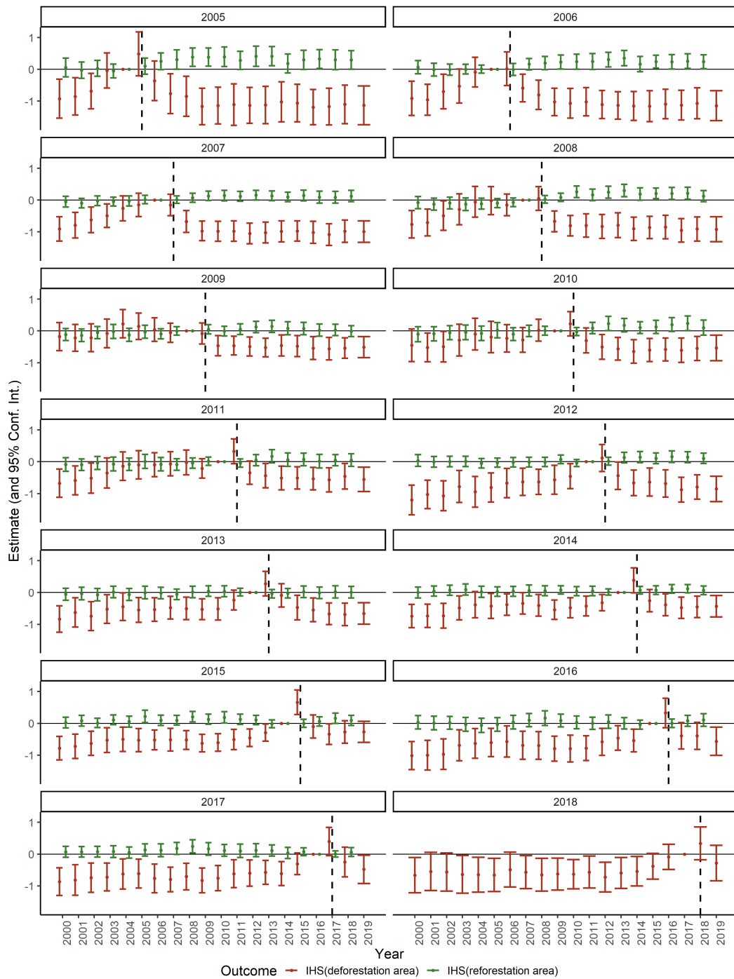
Figure A.4: Cohort-Time Direct Effects
