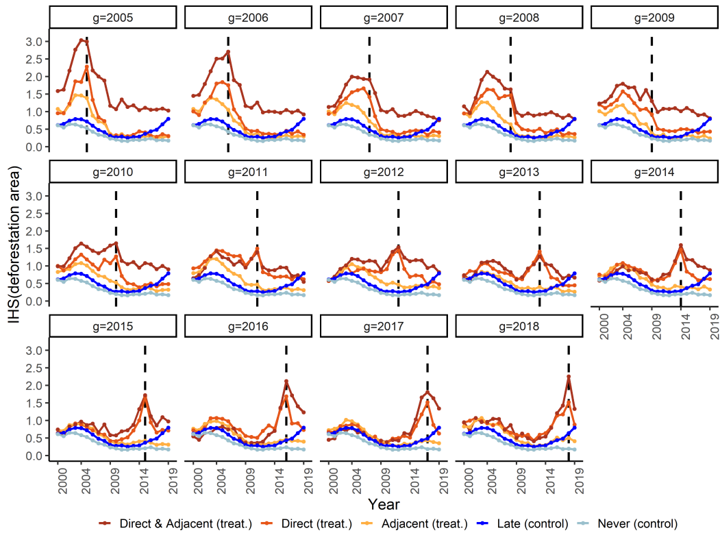
Figure 3.1: Deforestation Evolution by Punishment Type and Cohort
