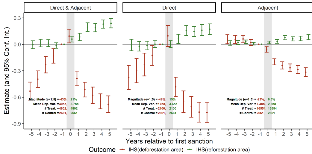
Figure A.7: Late-treated as Control Group
