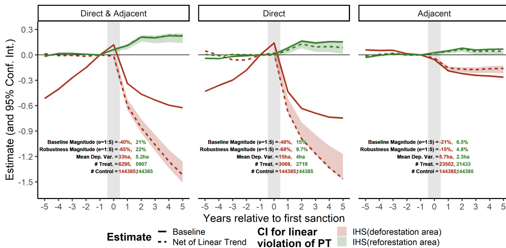
Figure 5.2: Robustness to Parallel Trends Violation
