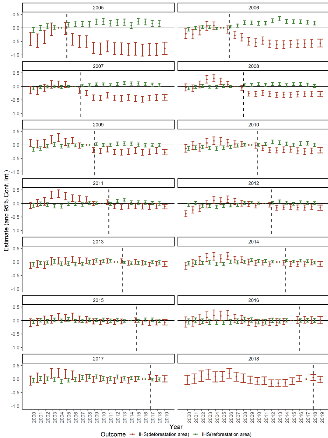
Figure A.5: Cohort-Time Adjacent Effects
