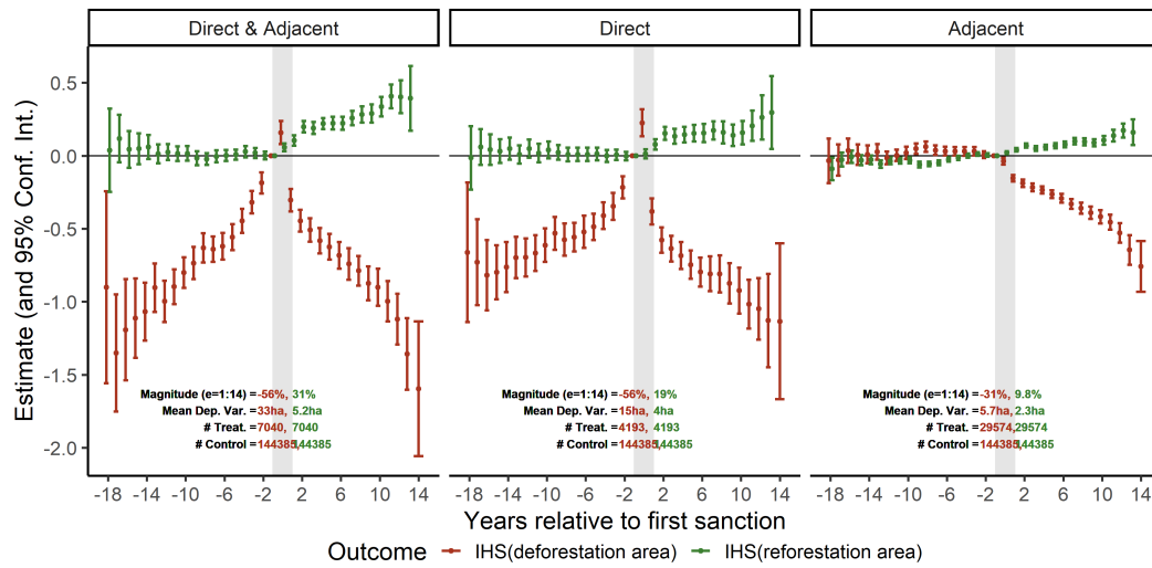
Figure A.6: Full Event-Study Estimates
