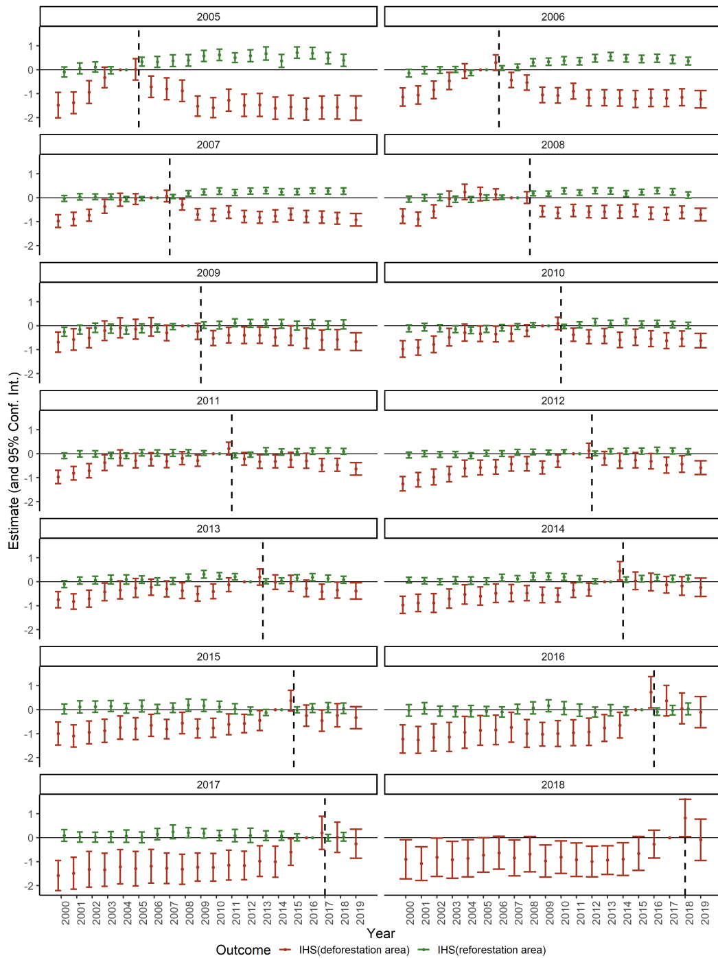
Figure A.3: Cohort-Time Direct & Adjacent Effects
