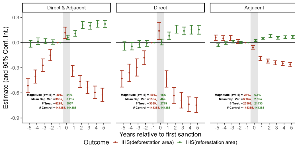
Figure 5.1: Sanction Effects on Deforestation and Reforestation
