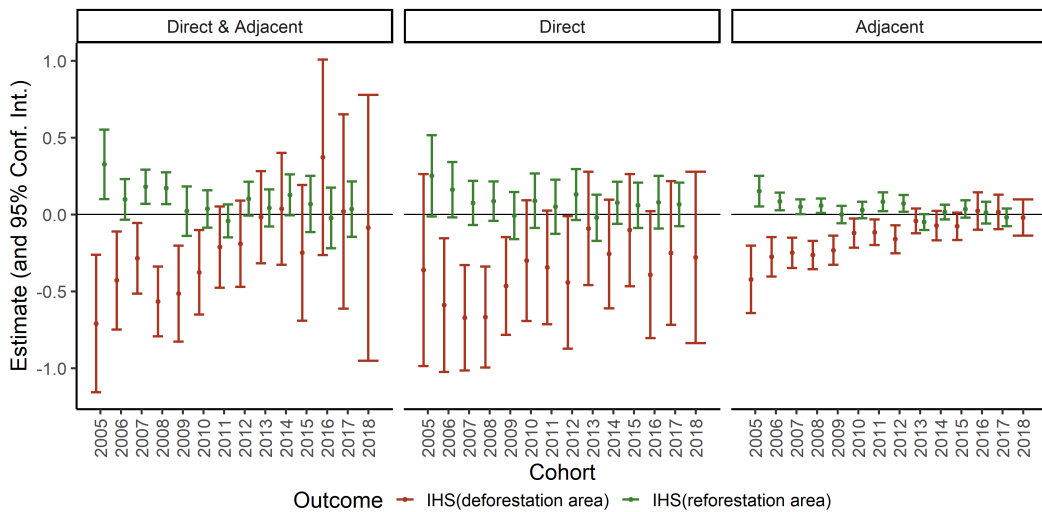
Figure 5.3: Sanctions Effects Over Time
