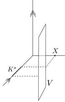
Figure 3.3: Vertical rectangle
