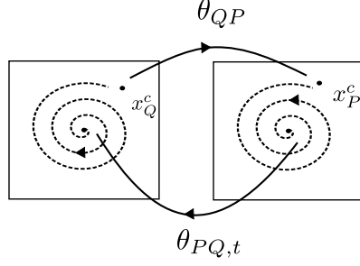
Figure 3.2: Quotient map
