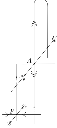
Figure 3.7: Perturbation
