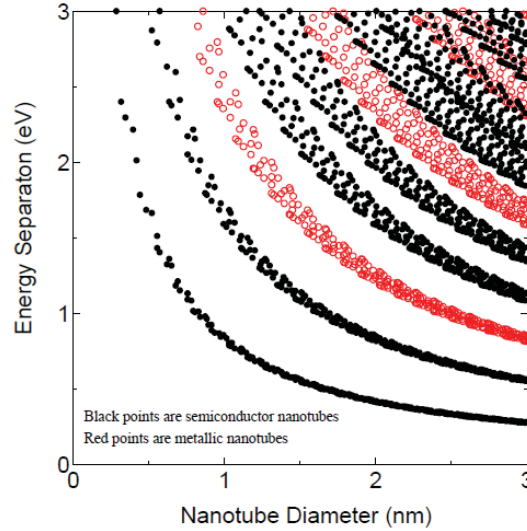
Figure 5.4: Katura plot from Dr. Prof. Shigeo Maruyama's page ( http://www.photon.t.u-tokyo.ac.jp/maruyama/index.html ).
