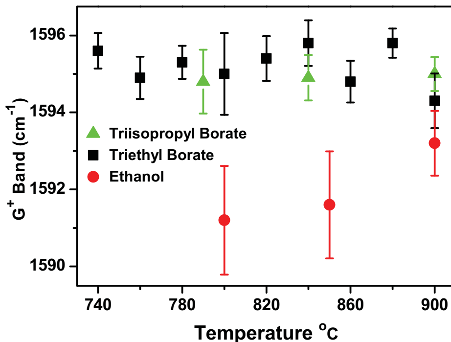
Figure 5.12: G^+ band position for different growing temperatures and precursors. Laser power used was around 0.13mW. The error bars are due to different points on the sample.
