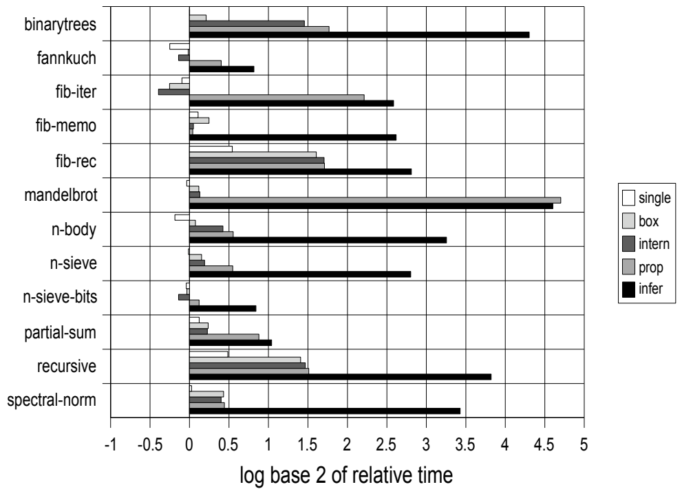
Figure 4.3: .NET 4.0 Beta 1 Comparison
