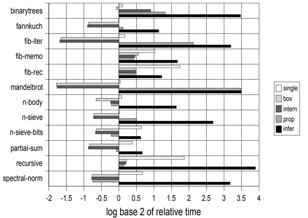
Figure 4.5: Mono 2.4 Comparison
