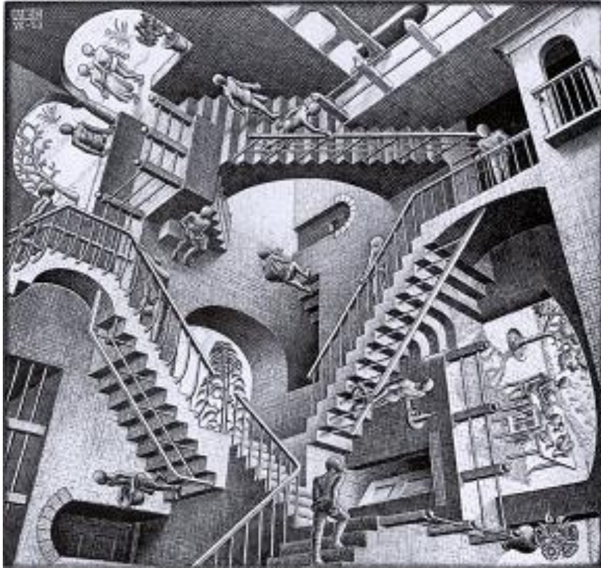
Escher, Relativity.
